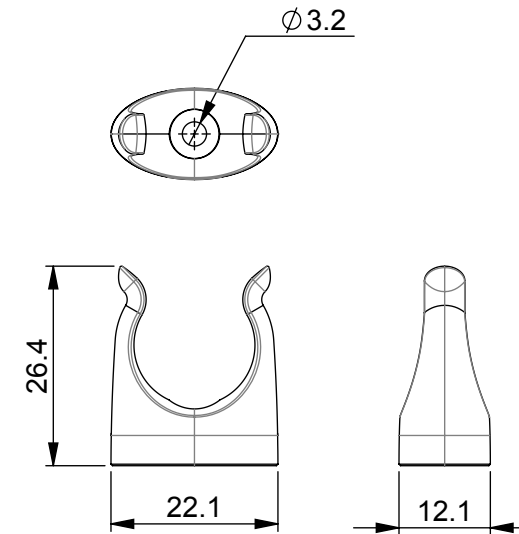
EJB-CLIP 16MM
